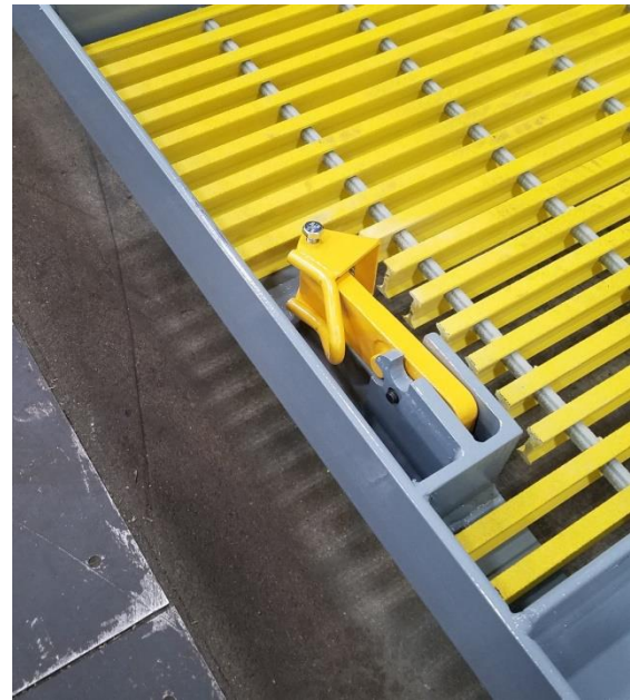
Non Slip Cat Walk and Vertical Restraint Stop
