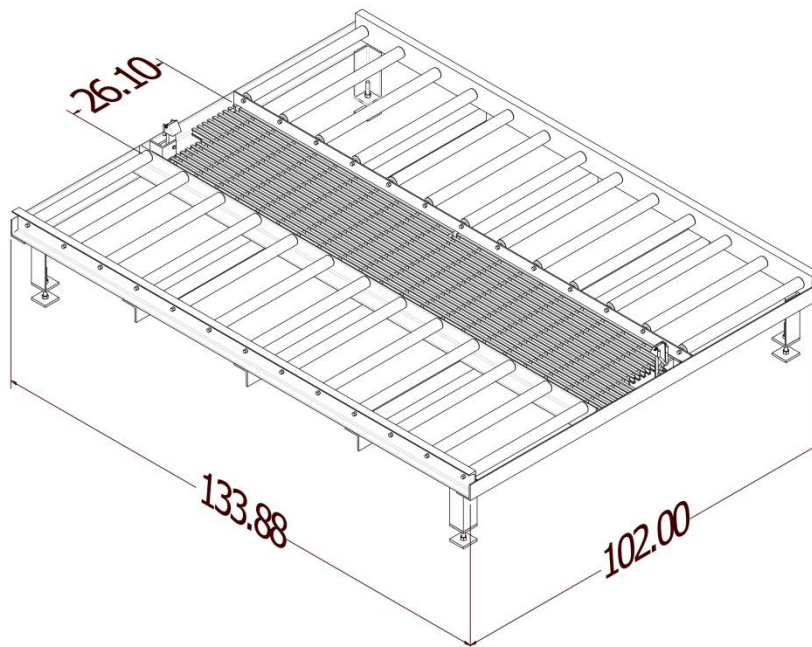
Overall Dimensions (inches) of MAXSON AVIATION Static Rack
